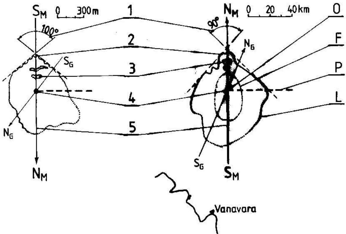
Fig. V5. The illustration of similarities existing between the configuration of the Tapanui Crater and that of the Tunguska blast site . The presence of such close similarities certify that the origin of both sites is analogous, i.e. from a powerful near-ground (aerial) explosion. Notice the evident correspondence (labelled 1 to 5) in: (1) the relationship between the apical angle of triangular entries to both sites and their distance from the nearest magnetic pole of Earth (i.e. at the moment of explosion the Tapanui Crater was located much closer to the magnetic pole than the Tunguska Site, thus its apical angle is also much wider), (2) the manner explosion shockwaves entered the ground, (3) the breaking points of the explosion shockwaves (which in Tunguska swirled tree trunks, whereas in Tapanui formed large sand dunes), (4) the location of the centre of explosions and the paths followed prior by both vehicles, (5) magnetic meridian orientation of the sites, etc. Symbols: S_G/N_G - geographic south-north direction, S_M/N_M - magnetic south-north direction.
