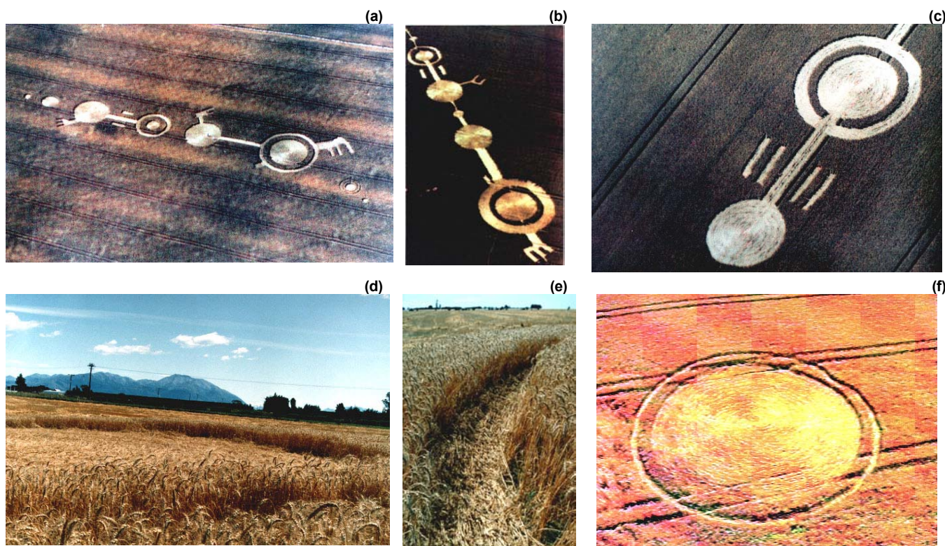
Fig. V3B. Examples of UFO landing sites made by flying clusters. They illustrate that the 'crop circles' are simply trails left by magnetic circuits of Magnocraft-type space vehicles (UFOs) hovering at low heights. To express the above in more simple terms, such circles are areas of vegetation immaculately "brushed down" and deformed by spinning streams of magnetic field force lines produced by propulsion system of UFOs which hovered just above this vegetation. Photographs (a) and (c) shown here appeared in the book [1FigV3] by Pat Delgado & Colin Andrews, "Crop Circles - the Latest Evidence" (Bloomsbury Publishing Limited, 2 Soho Square, London W1V 5DE) 1990, ISBN 0-7475-0843-7, pages 45 & 59.
