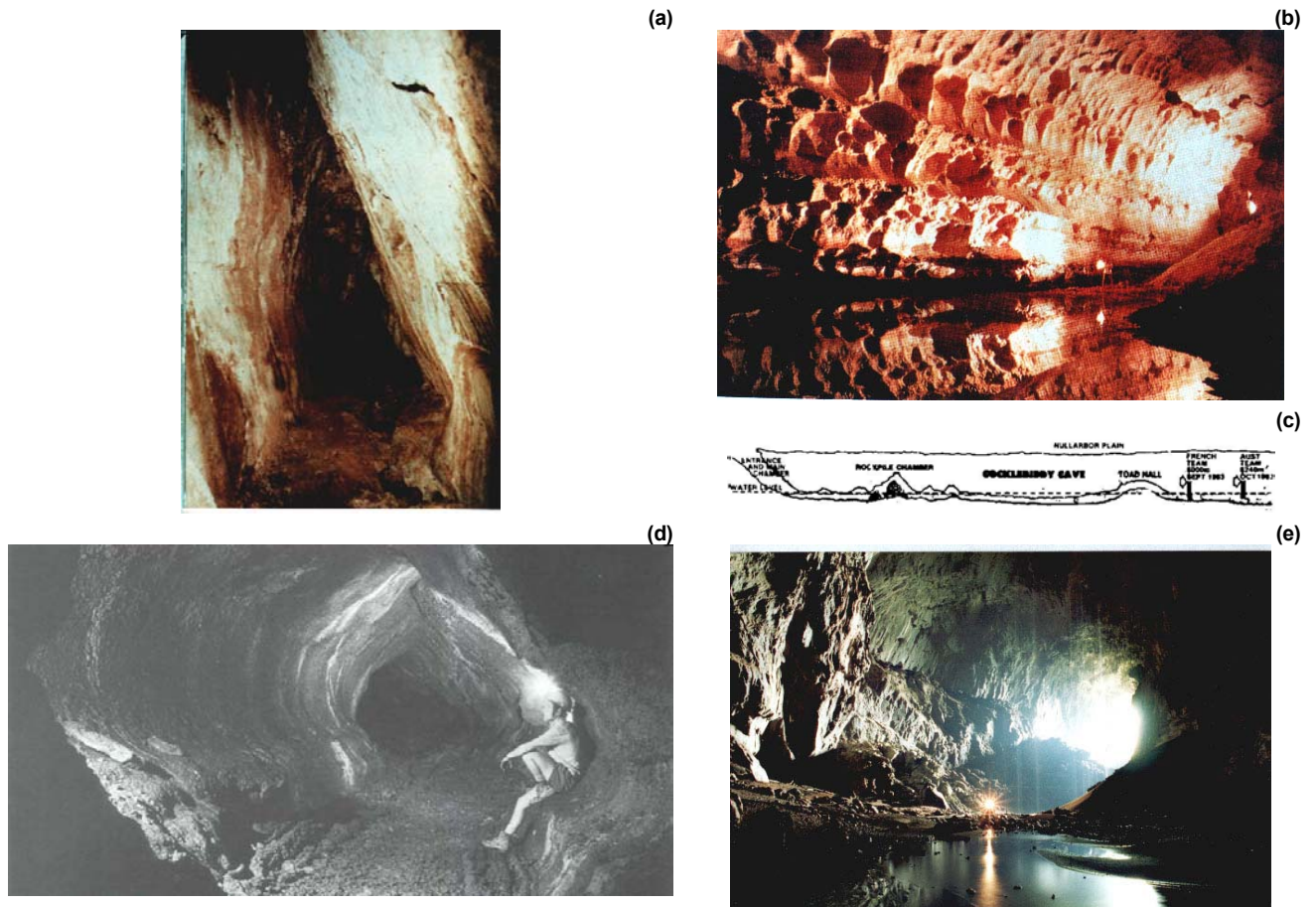
Fig. V6. Smooth, long, straight, geometrically shaped, and magnetized tunnels made during underground flights of UFOs. Principles involved in the formation of such tunnels, explained by the Theory of the Magnocraft and illustrated as if the ground were transparent, are shown in Figure F31. Their final shape (i.e. elliptical or triangular) results from the requirement that the base of a saucer-shaped Magnocraft must all times remain perpendicular to the force lines of the local magnetic field.
