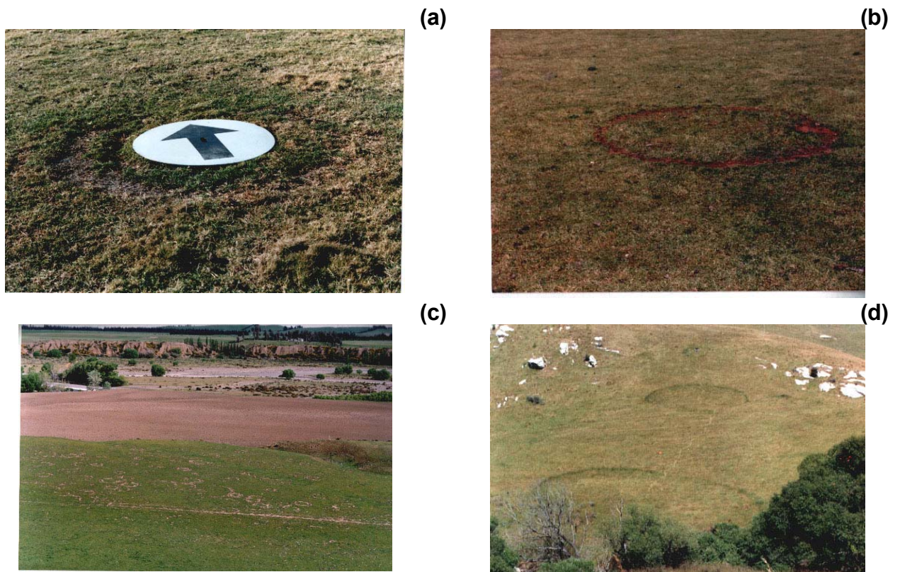
Fig. V1. Photographs of landing sites formed by single UFOs , which illustrate all three main cases presented in Figure F38 (a-c).
